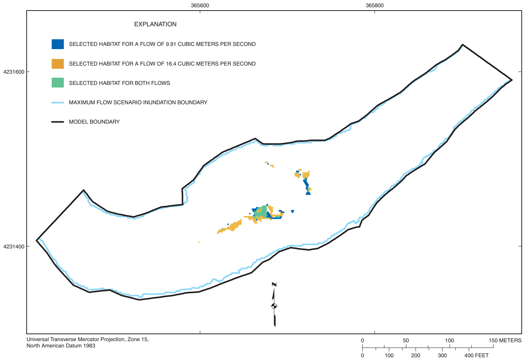
Figure 4-72. Selected habitat area distribution for habitat category 19 (stonecat) at flows of 9.91 and 16.4 cubic meters per second at Marais des Cygnes River site MDC2.
